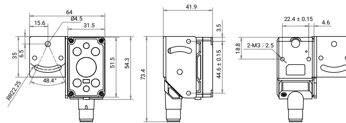
Device and Installation Bracket 1 (Straight Angle)
