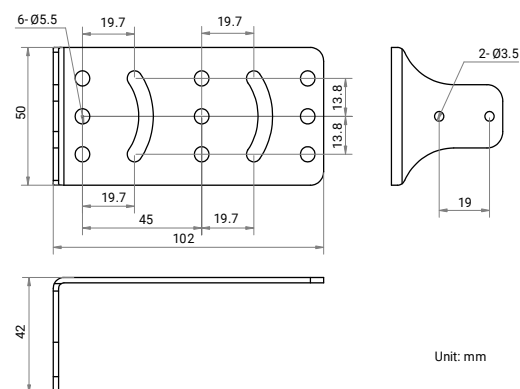
Installation Bracket:
