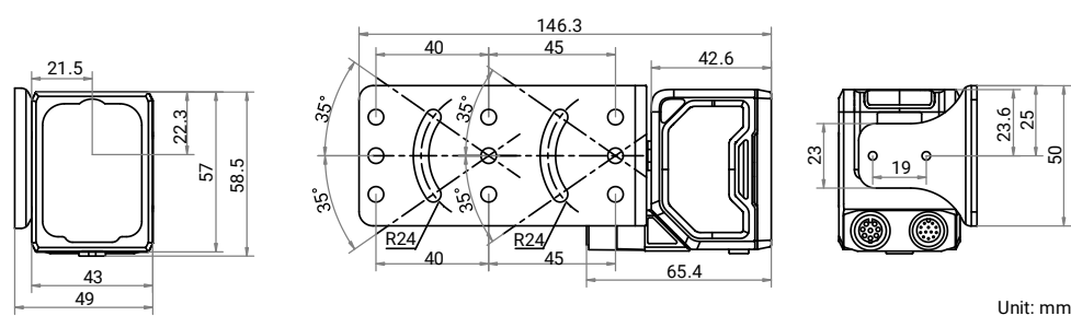
Device and Installation Bracket (Right Angle):
