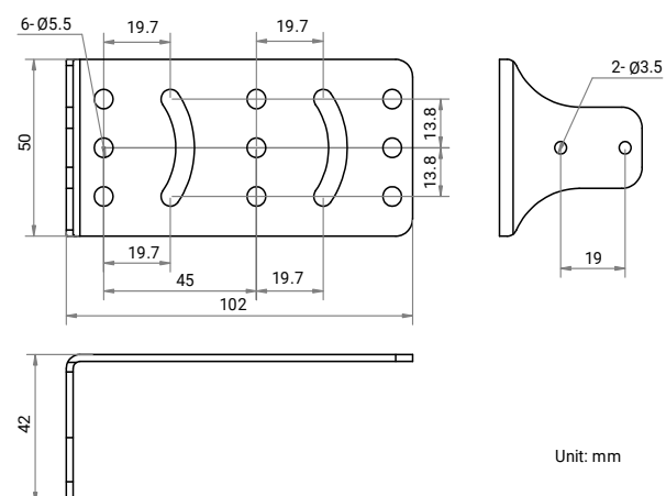
Installation Bracket:
