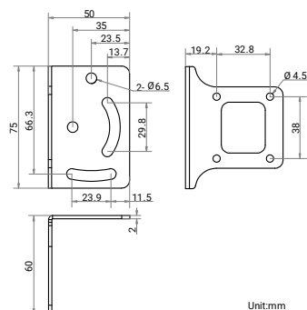
Installation Bracket:
