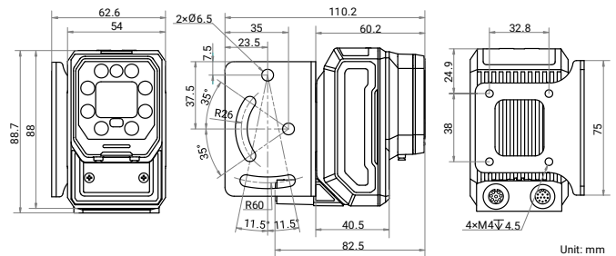
Installation Bracket:
