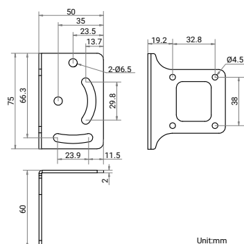
Installation Bracket:
