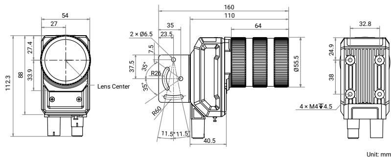
Device and Installation Bracket (Right Angle):
