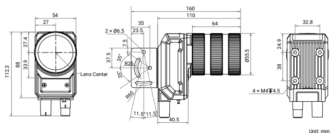
Device and Installation Bracket (Right Angle):
