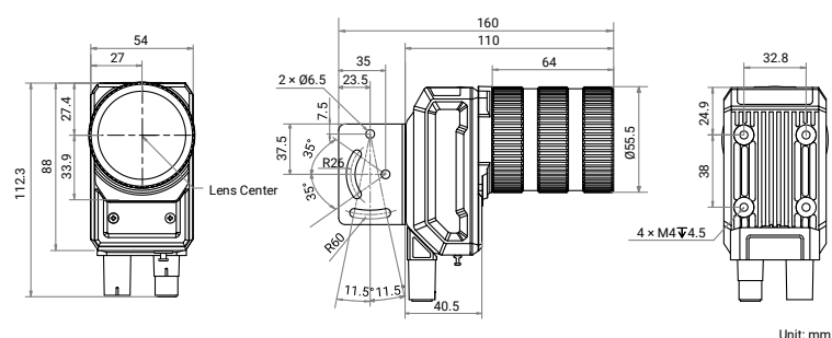
Device and Installation Bracket (Right Angle):
