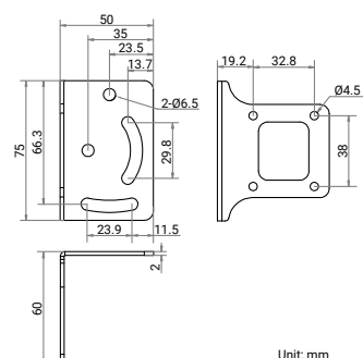
Installation Bracket:
