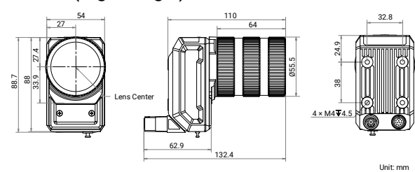
Device (Right Angle):
