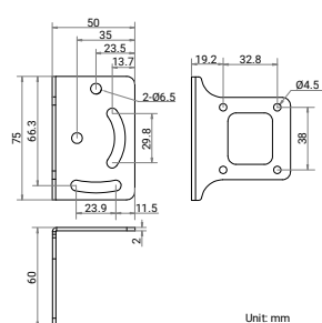
Installation Bracket:
