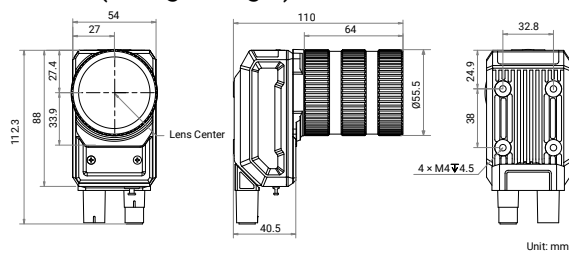
Device and Installation Bracket (Straight Angle):
