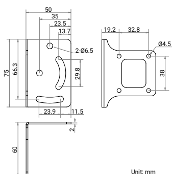
Installation Bracket:
